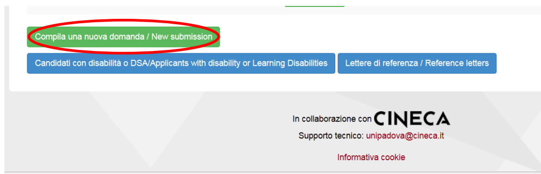
Fig. 4 – New submission
