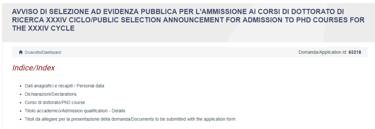
Fig. 5 – Application Sections
